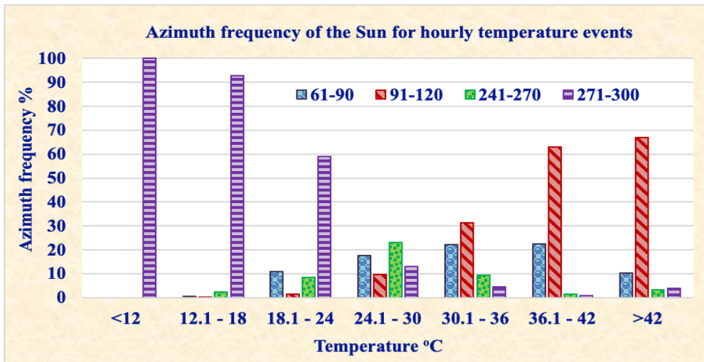
Fig. 3. Azimuth frequency of the Sun for temperature events
