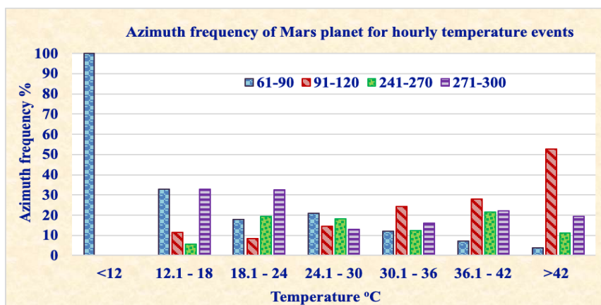
Fig. 7. Azimuth frequency of Mars planet for temperature events
