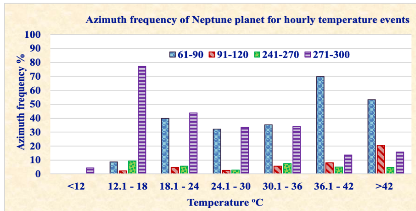
Fig. 11. Azimuth frequency of Neptune planet for temperature events
