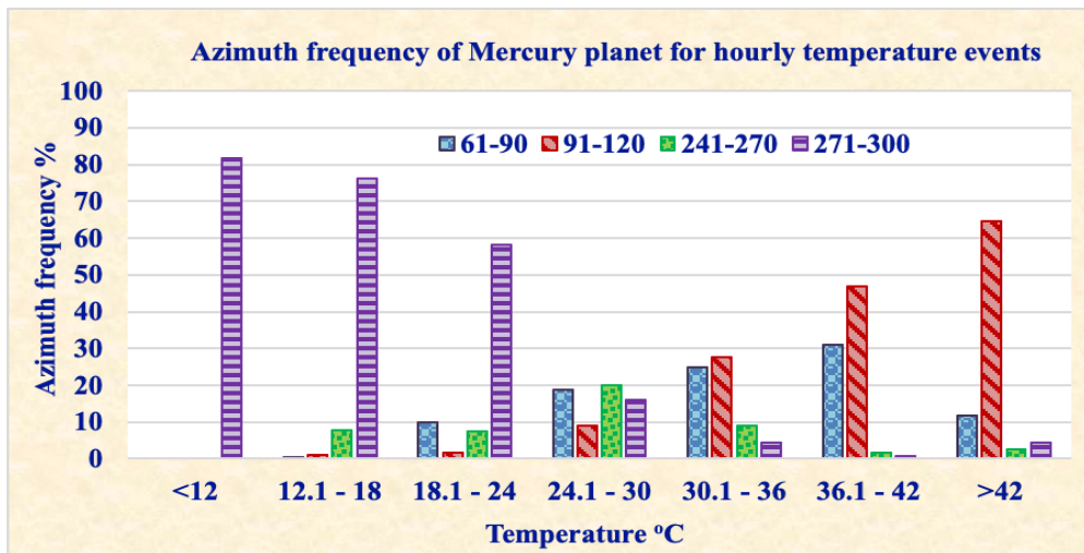
Fig. 4. Azimuth frequency of Mercury planet for temperature events
