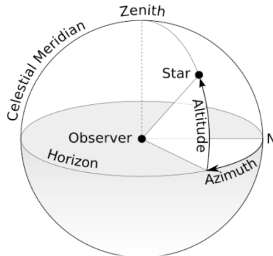
Fig. 2. Calculating azimuth of the celestial body from the observer location
