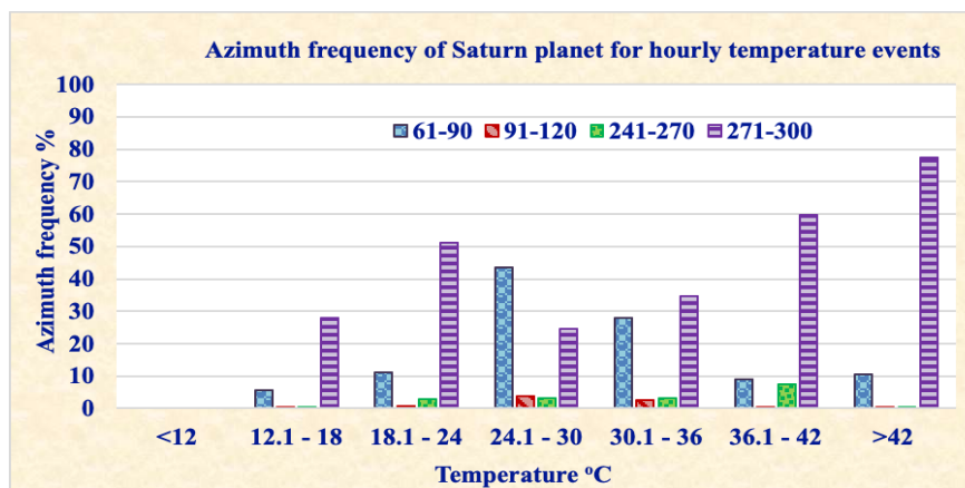
Fig. 9. Azimuth frequency of Saturn planet for temperature events
