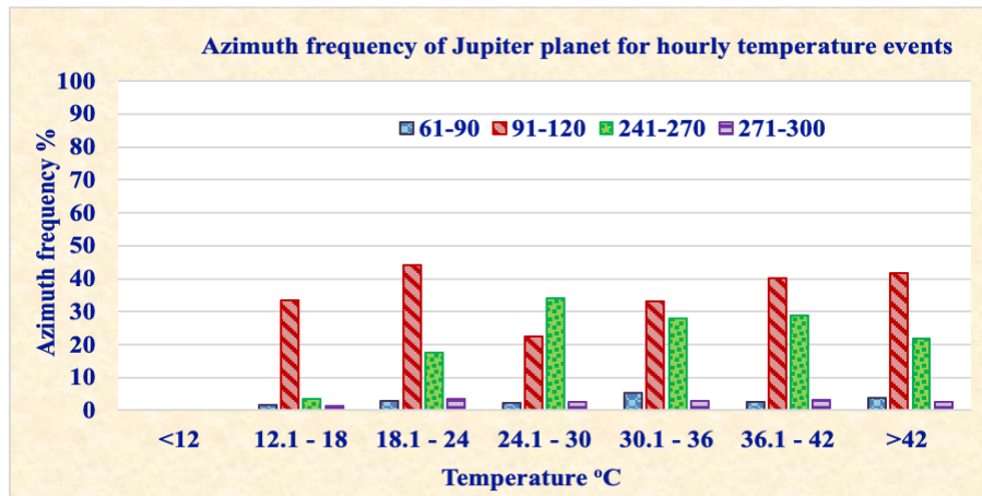
Fig. 8. Azimuth frequency of Jupiter planet for temperature events
