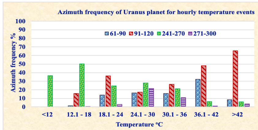
Fig. 10. Azimuth frequency of Uranus planet for temperature events
