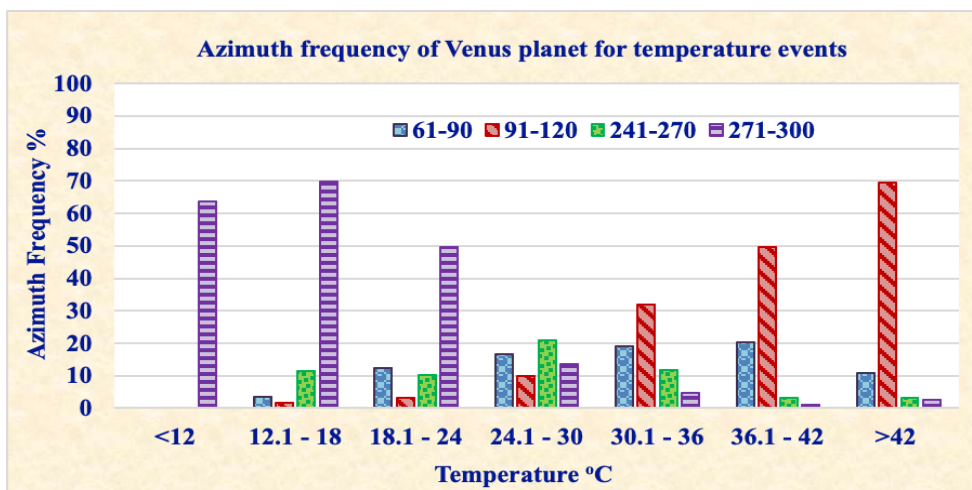
Fig. 5. Azimuth frequency of Venus planet for temperature events
