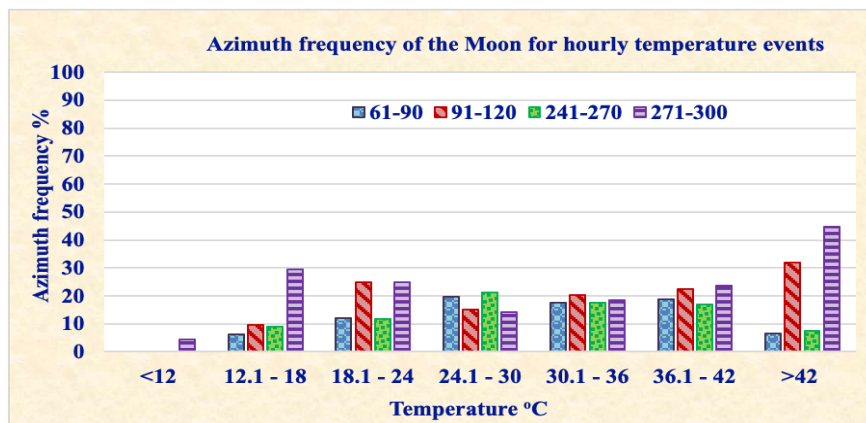
Fig. 6. Azimuth frequency of the Moon for temperature events
