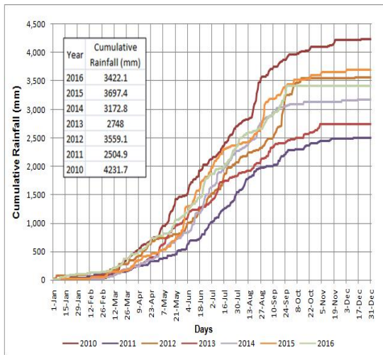
Fig. 5. Yearly cumulative rainfall during 2010 – 2016
