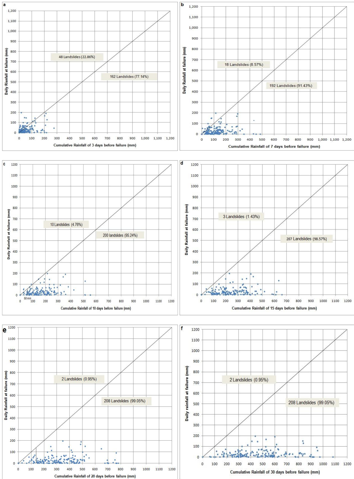
Fig. 12.a – f. Relation between antecedent rainfall prior to failure (3, 7, 10, 20 and 30 days) and daily rainfall for landslide occurrences
