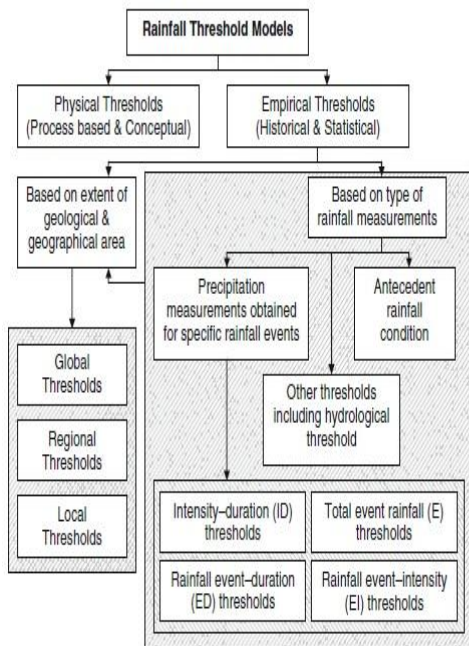
Fig. 3. Different rainfall threshold models for landslide occurrences (Kanungo 2013)
