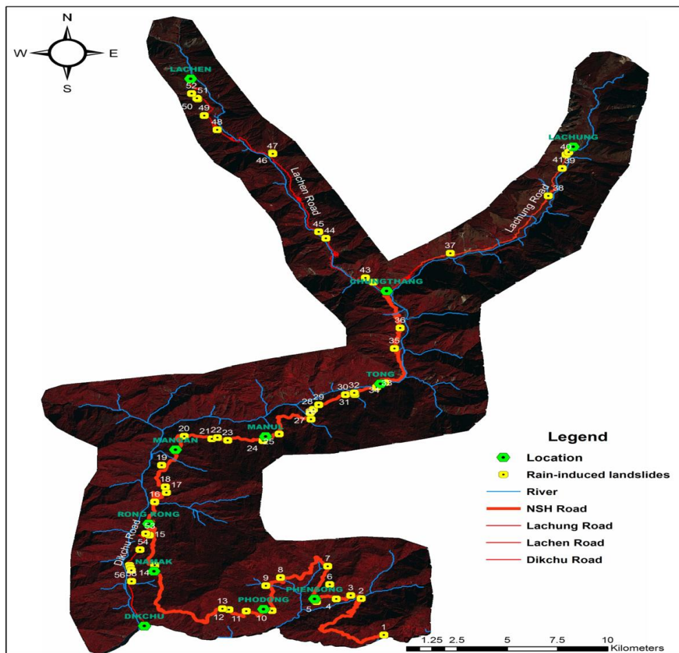
Fig. 7. Location of the major rain – induced landslide in North Sikkim road corridor (study area)
