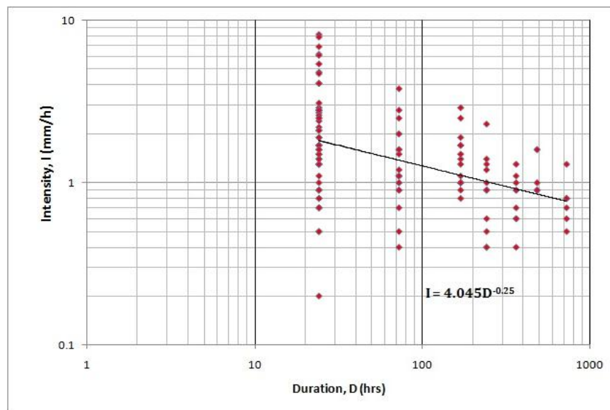
Fig. 9. Rainfall Intensity–Duration (ID) threshold based on estimation from daily rainfall data for the initiation of landslides in north Sikkim road corridor of Sikkim Himalaya, India
