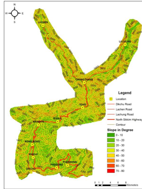
Fig. 2. Slope map of the study area
