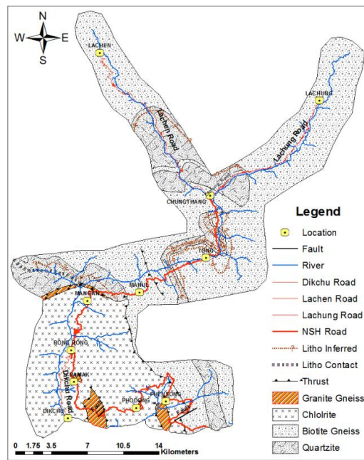
Fig. 4. Geological condition of the study area
