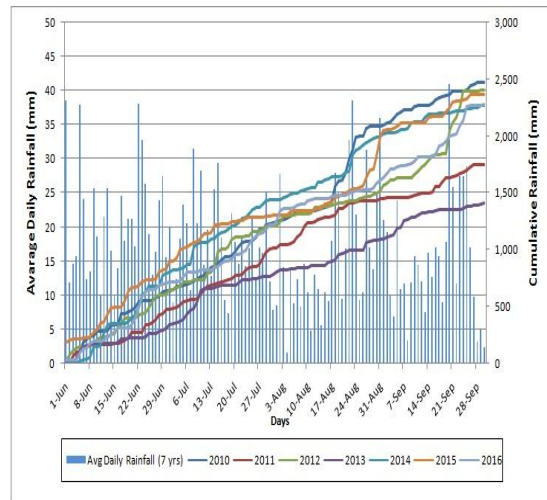
Fig. 6. Average daily rainfall and cumulative rainfall during the monsoon from 2010 – 2016
