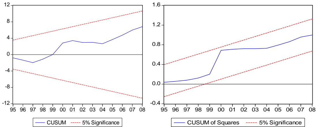
Fig. 2. Plot of both the CUSUM and CUSUM squared tests for the dependent variable IY.
